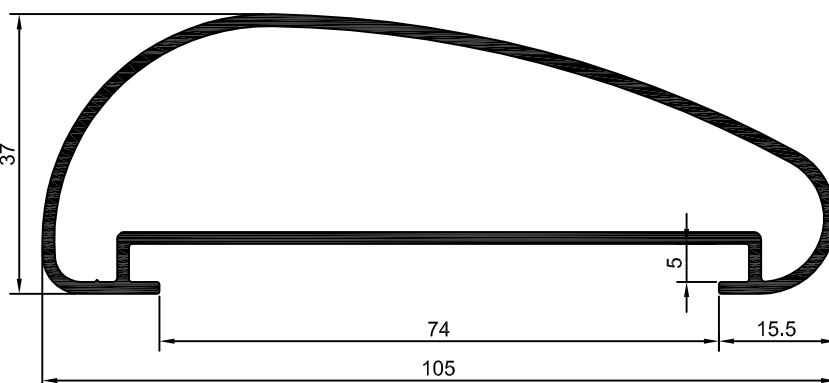
GR-020 1,138 Kg/m
