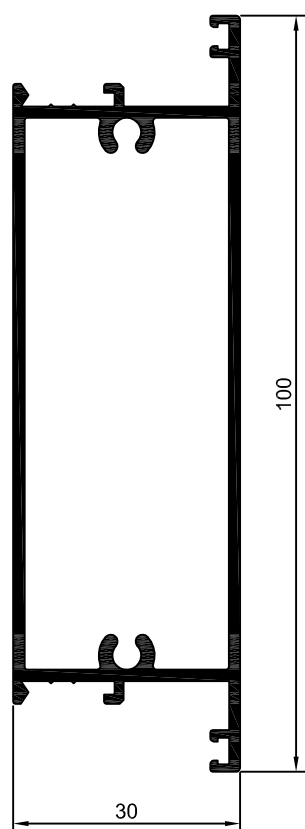
30-030 30-030 1,114 Kg/m
