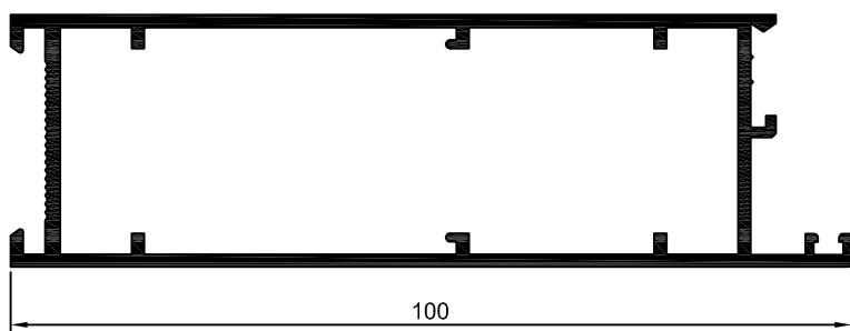
30-082 30-082 1,130 kg/m
