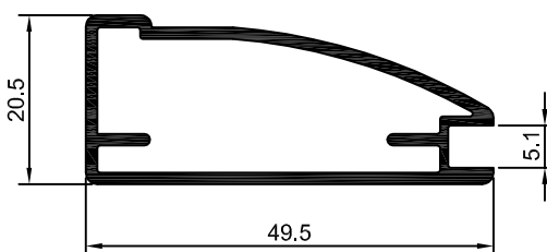
MV-011 0,542 Kg/m
