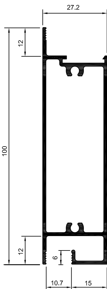
30-016 ME-078 1.045 Kg/m
