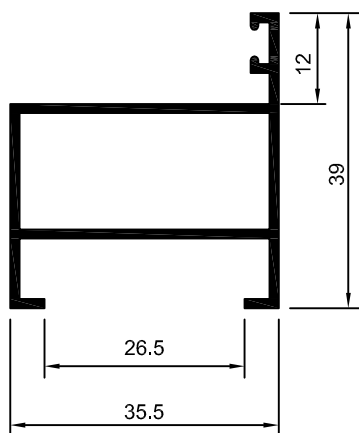
30-013 ME-073 0.470 Kg/m
