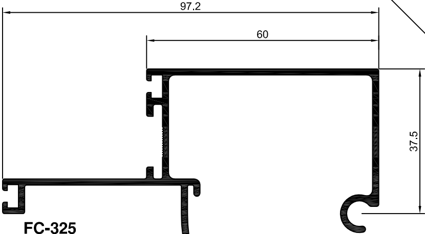
FC-325 FC-325 1,163 Kg/m
