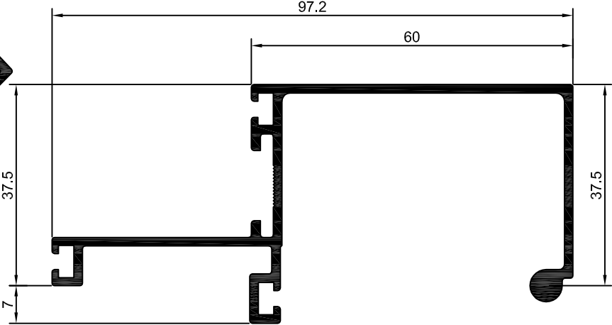
FC-326 FC-326 1,016 Kg/m
