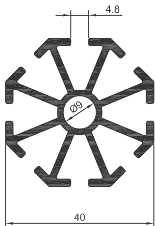
DS-255 1,096 Kg/m
