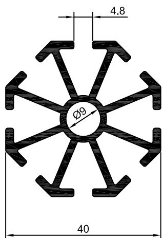
DS-255 1,096 Kg/m
