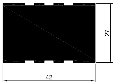
DS-527 2,992 Kg/m
