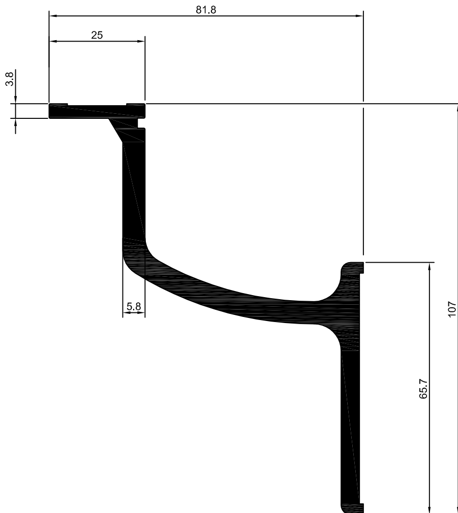
DS-838 2,225 Kg/m
