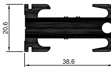
DS-823 1,222 Kg/m
